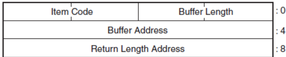
Figure 11.4. Item_list_3 Format
