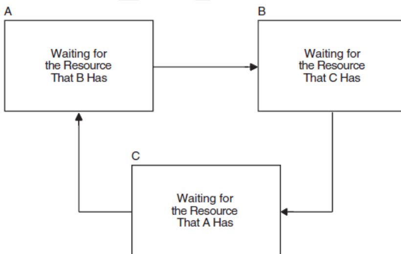
Figure 7.3. Deadlock
