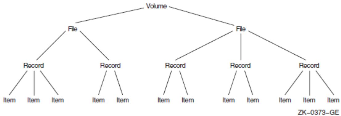
Figure 7.1. Model Database
