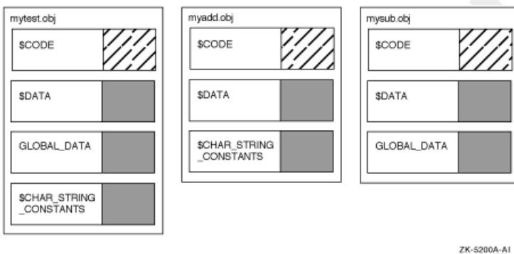
Figure 7.2. Program Sections Created for Examples 3-1, 3-2, and 3-3
