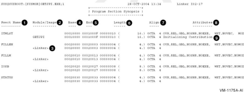
Figure 5.1. Program Section Synopsis
