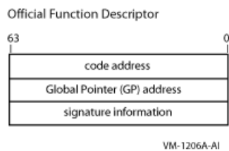
Figure 3.3. Official Function Descriptor
