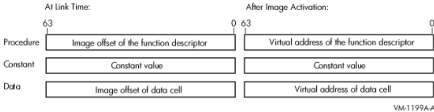
Figure 2.1. Symbol Vector Contents
