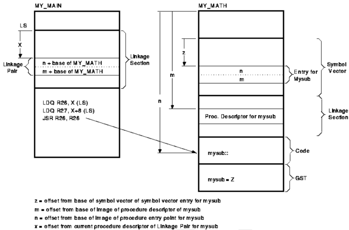
Figure 4.1. Accessing Universal Symbols Specified Using the SYMBOL_VECTOR=Option
