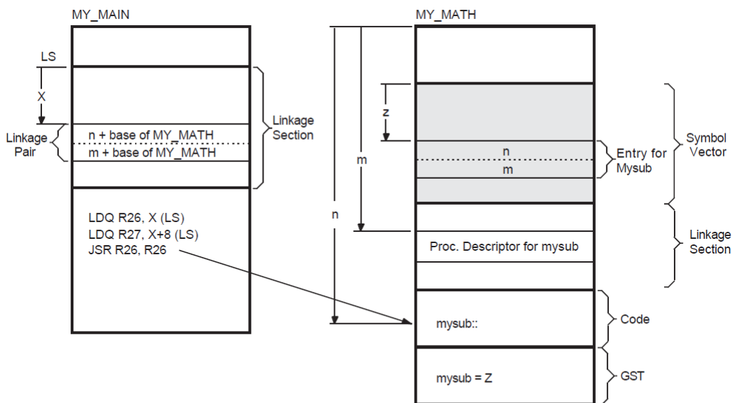
Figure 8.2. Accessing Universal Symbols Specified Using the SYMBOL_VECTOR=Option
