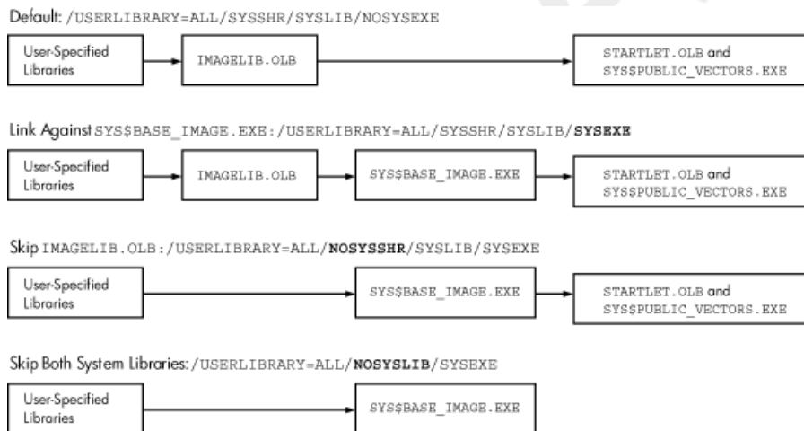
Figure 2.4. Linker Processing of Default Libraries and SY$BASE_IMAGE.EXE
