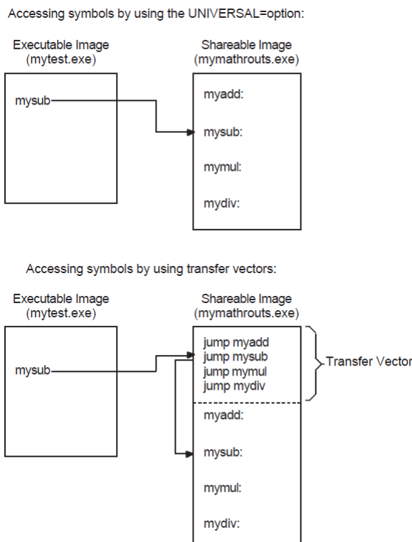
Figure 8.1. Comparison of UNIVERSAL= Option and Transfer Vectors
