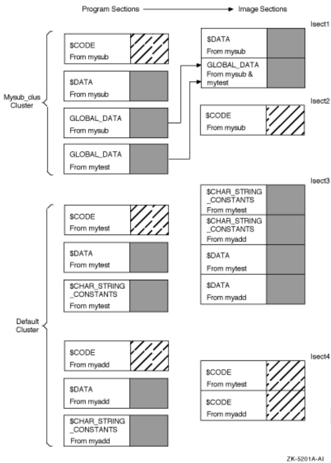
Figure 7.3. Combining Program Sections into Image Sections
