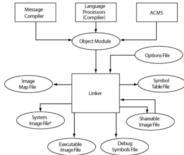
Figure 1.1. Position of the Linker in Program Development
