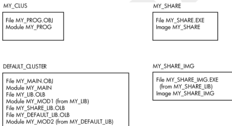
Figure 2.3. Clusters Created for Sample Link
