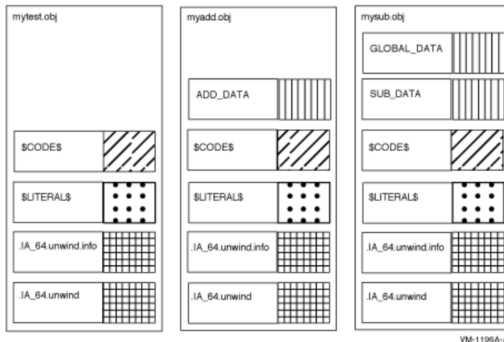
Figure 3.2. Sections Created for Examples 3-1, 3-2, and 3-3
