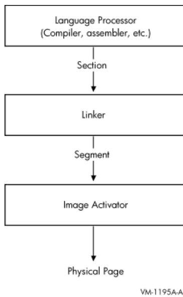
Figure 3.1. Communication of Image Memory Requirements on I64 Systems
