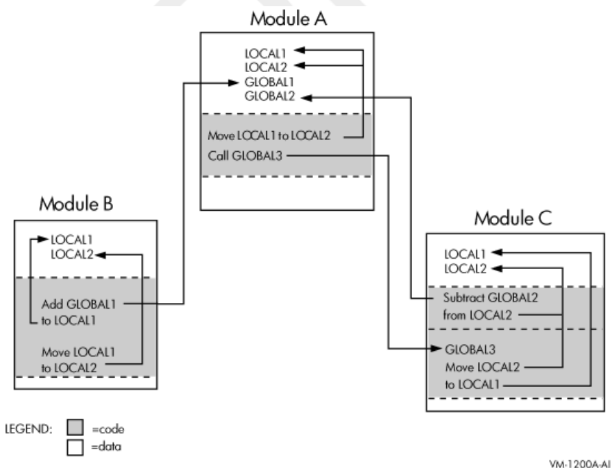
Figure 2.2. Symbol Resolution
