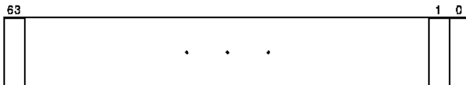
Figure 10.3. Vector Mask Register (VMR)
